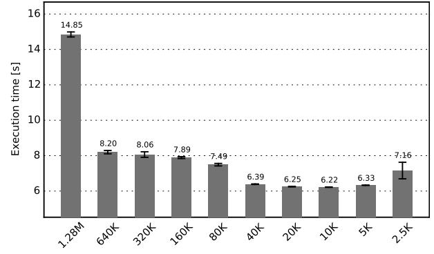
Fig. 12: K-means : execution time as a function of block size
