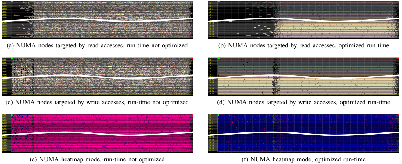
Fig. 14: Seidel: locality of memory accesses
