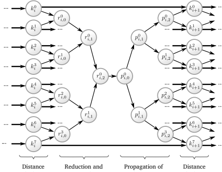
Fig. 11: Excerpt of the task graph for k-means
